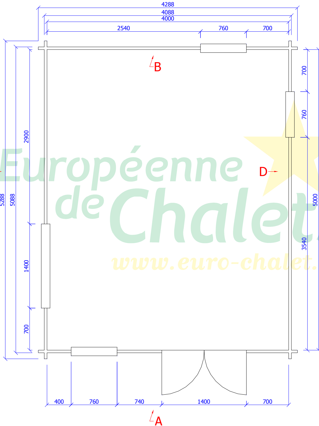
Plan
